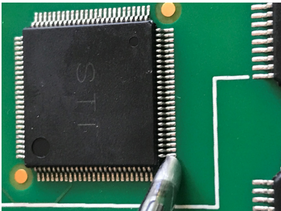
Figure 5. The quality of solder joints typically meet IPC Class 3 inspection criteria.
